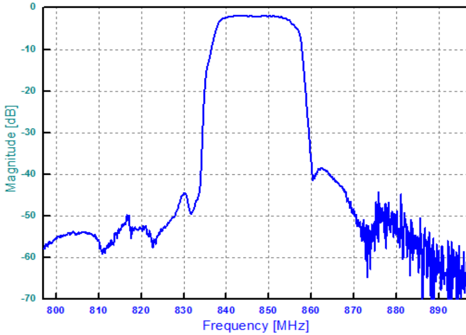
Frequency Response
